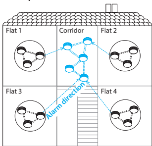
Fig. 16 Example of shared radio group
