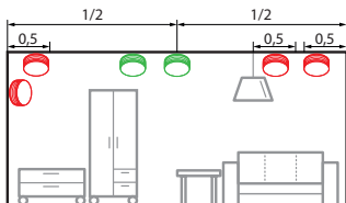
Fig. 11 Rooms with straight ceilings
