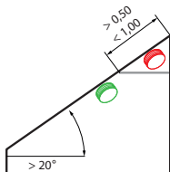
Fig. 12 Rooms with slanted ceilings
