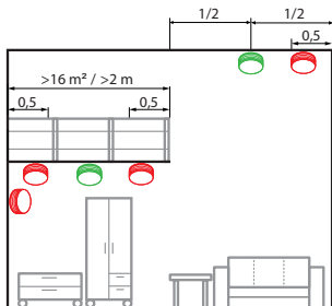
Abb. 15 Rooms with a platform or gallery
